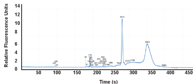
Figure 6: Electropherogram of HeLa Total RNA replicate 1 (see Figure 1, lane2).
